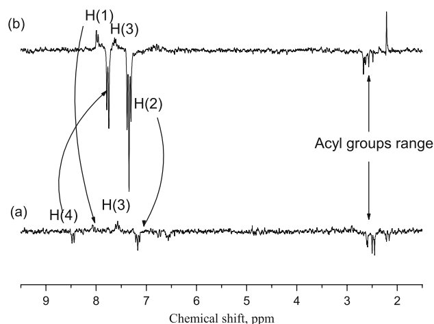
Fig. 2 1 H photo-CIDNP spectra of 1 mM of MA3 in D 2 O/CD 3 OD mixtures with \varphi : (a) 0 and (b) 0.8
