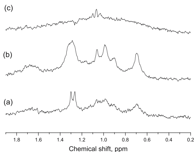
Fig. 5 1 H NMR spectra of CH 3 groups of GA in the D 2 O/CD 3 OD ( \varphi = 0.8 ) at the different concentrations GA: (a) 0.5 mM, (b) 1.0 mM, (c) 1.5 mM
