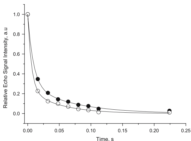
Fig. 6 Spin echo intensity dependences on time of \text{CH}_3 protons of GA at different concentrations (●) 0.25 mM and (○) 1 mM in \text{D}_2\text{O}/\text{CD}_3\text{OD} mixture ( \varphi = 0.8 ). Solid lines corresponds the best fitting curves
